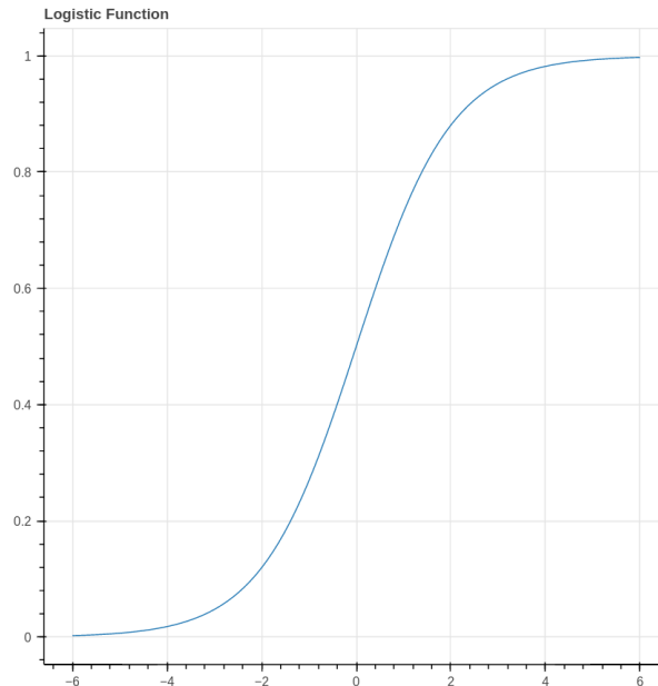
Figure 6.1: Logistic Curve
