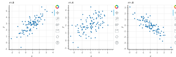
Figure 2.1: Correlation
