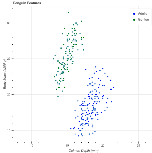
Figure 7.1: Penguin Scatterplot
