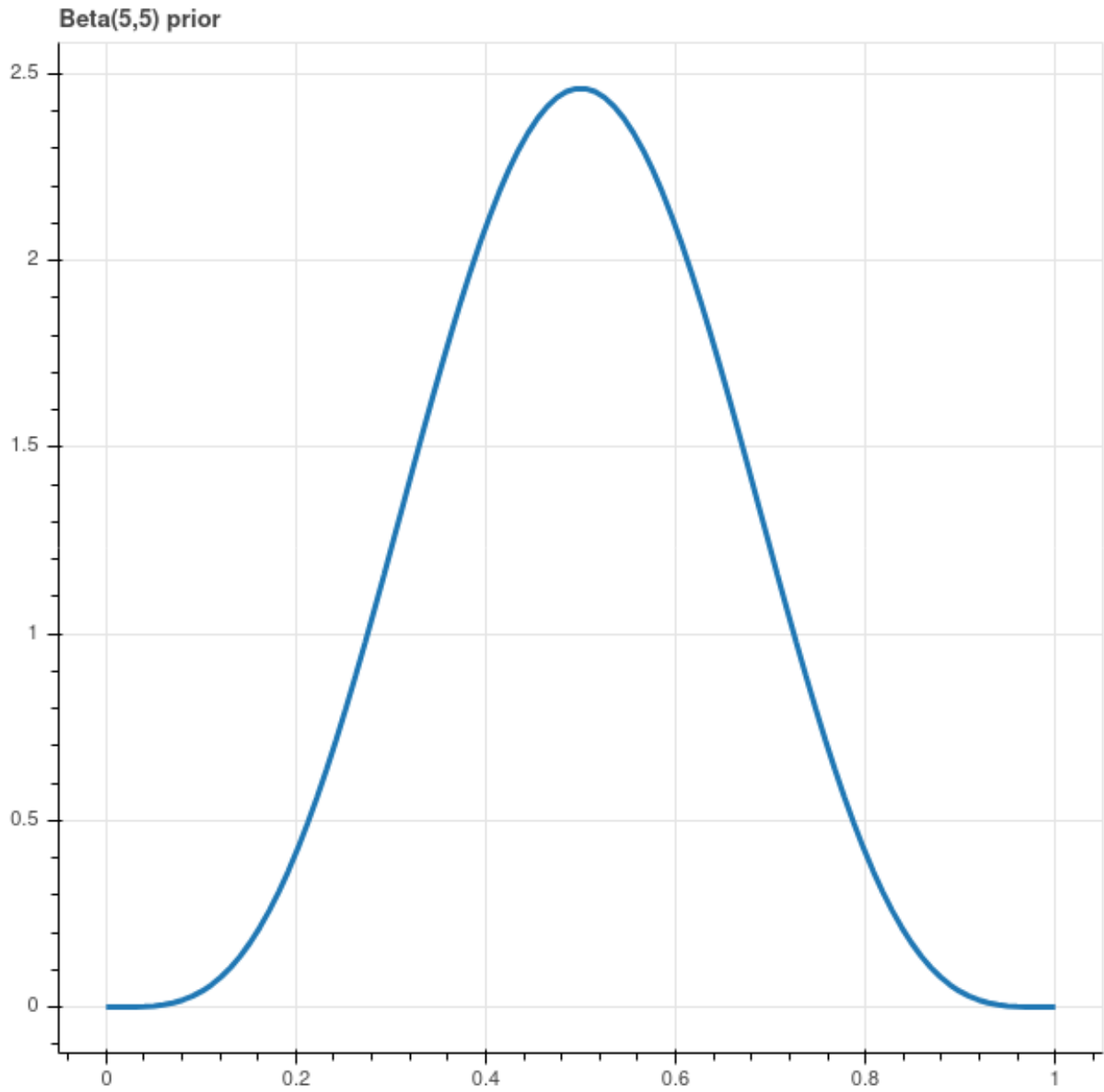
Figure 3.9: Beta(5,5) Prior
